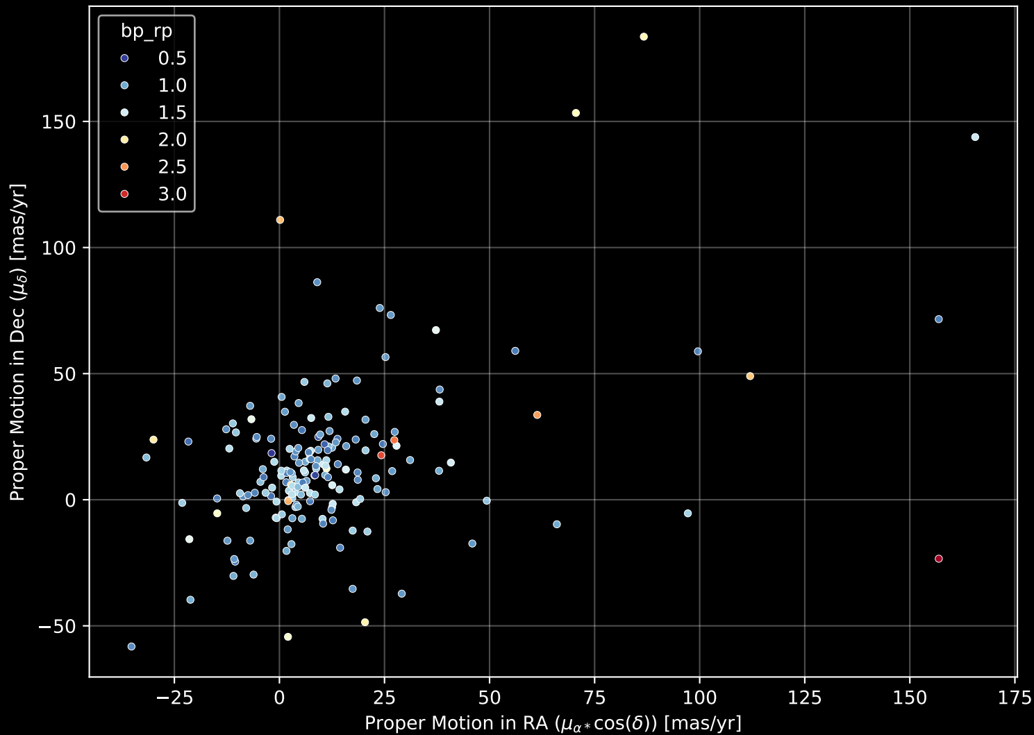
APOGEE DR17 Field: [286-36-O_TESS] Proper Motion Diagram (n= 182)
