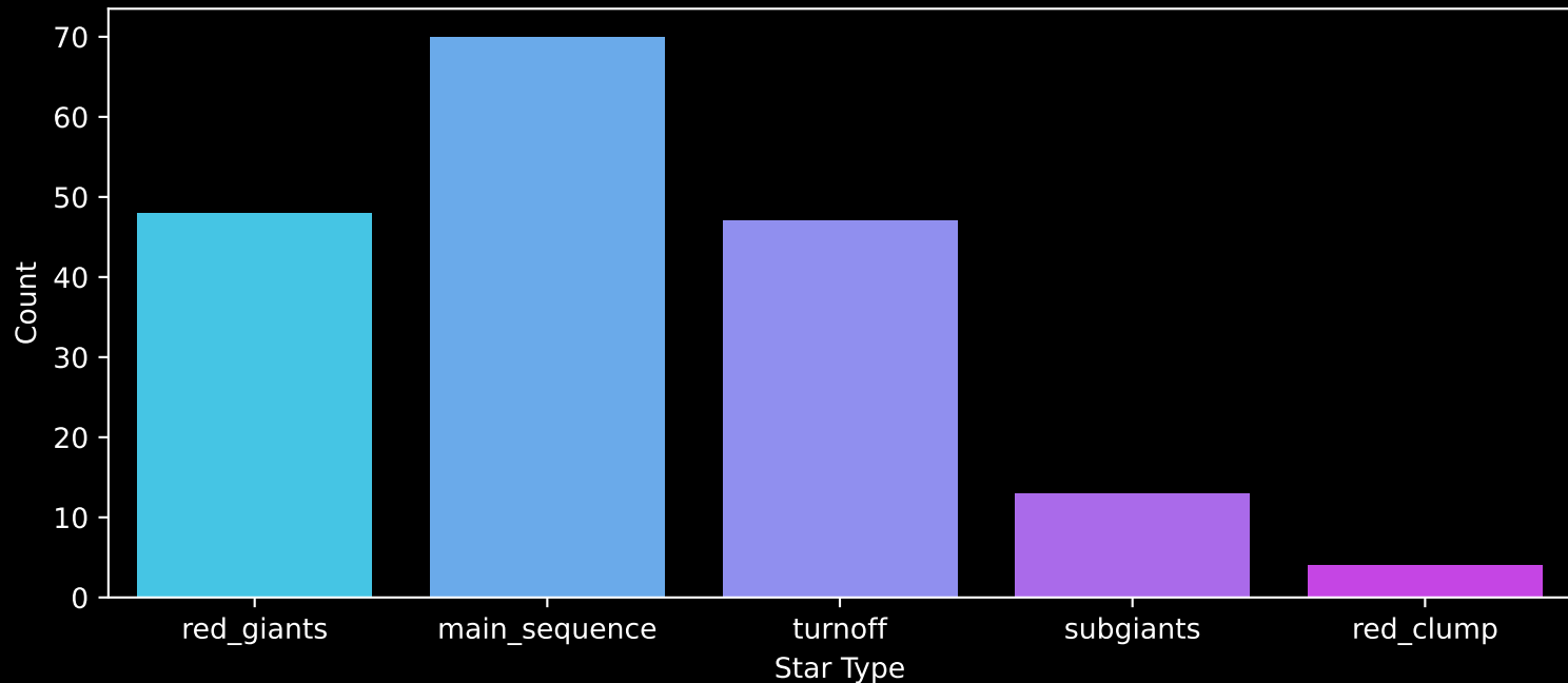
APOGEE DR17 Field: [286-36-O_TESS] Count plot of Star Type
