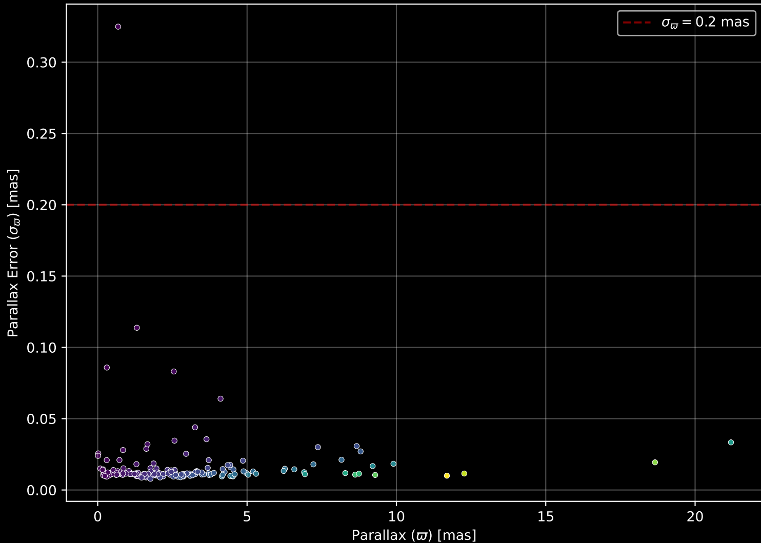
APOGEE DR17 Field: [286-36-O_TESS] Parallax Quality (n= 182)
