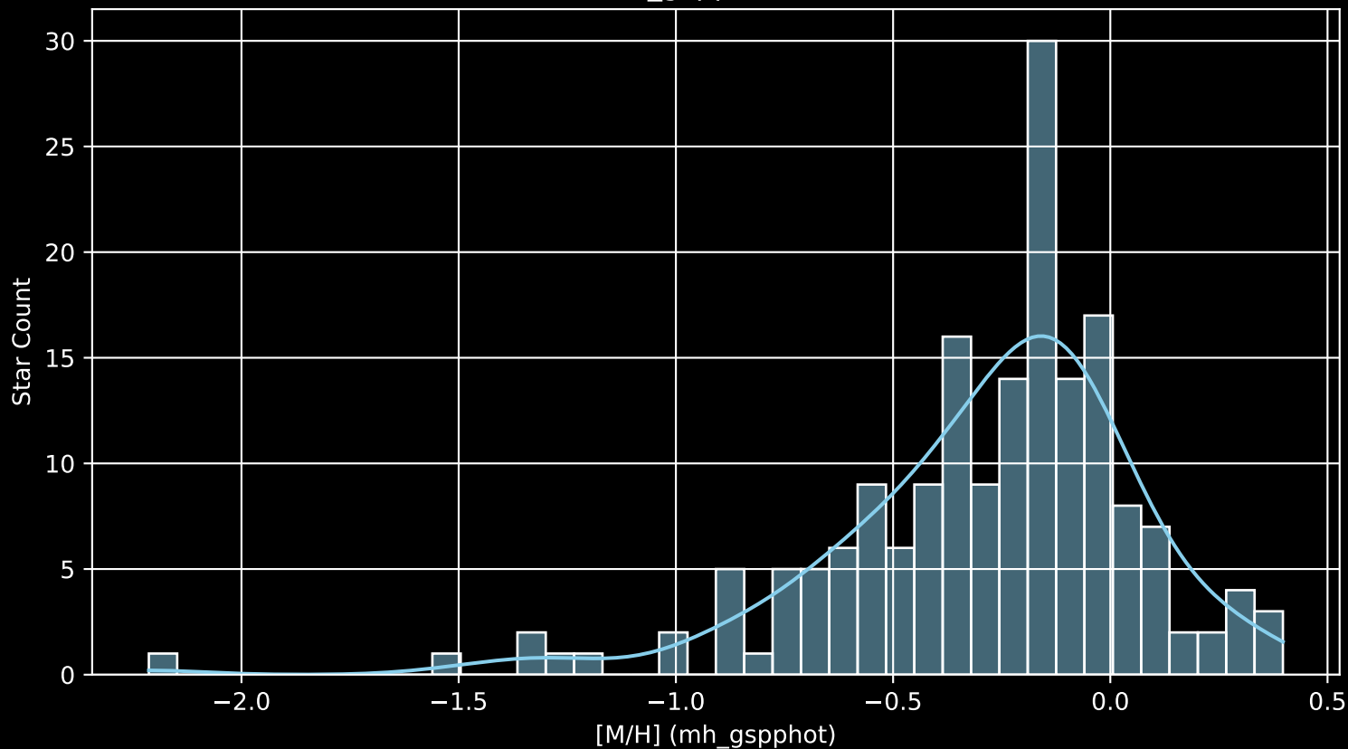
APOGEE DR17 Field: [286-36-O_TESS [M/H] (mh_gspphot) (n= 180)
