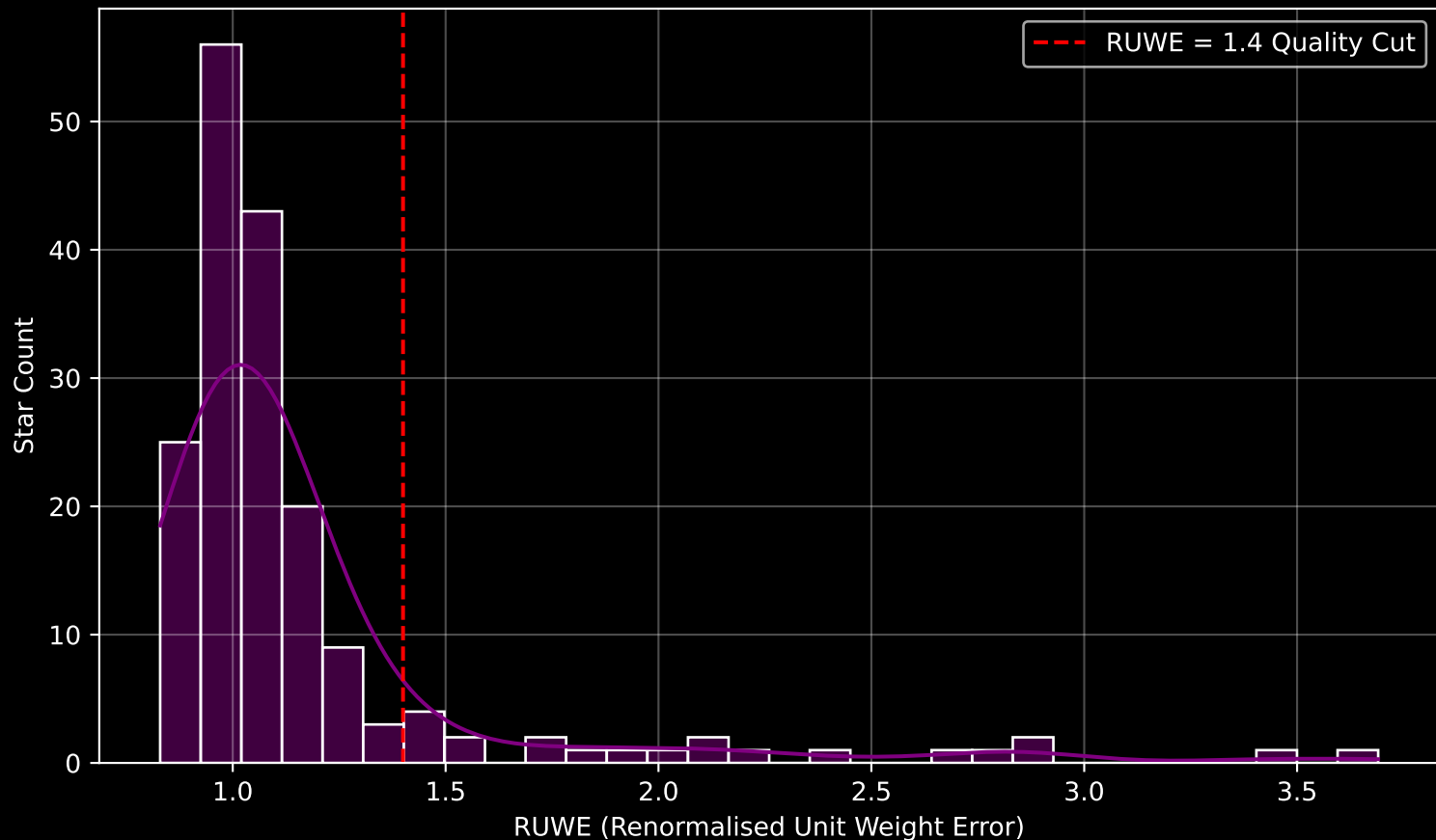
GAPOGEE DR17 Field [286-36-O_TESS] RUWE Distribution (n= 177)
